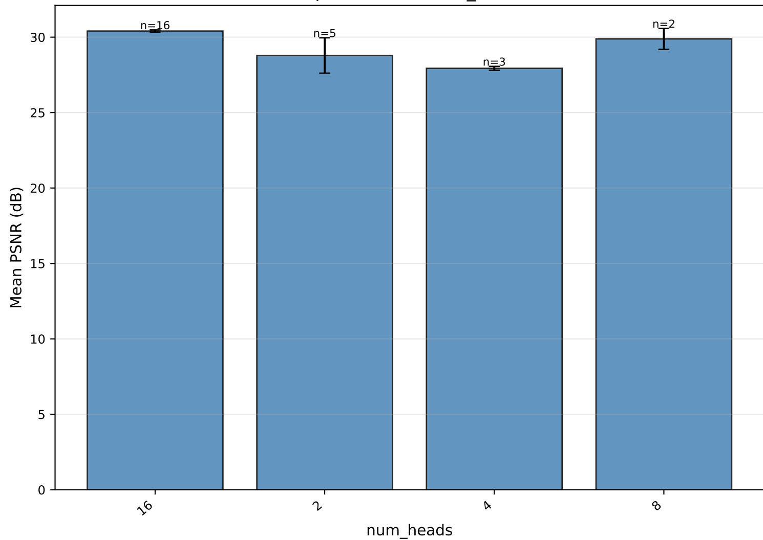
Mean PSNR per value of num_heads — SwinT
